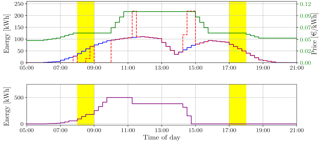
Fig. 2. Results for Entity 1 on day 24 under Problem 1. Energy production forecast \hat{E}_a(t) (blue), sold energy E_s^e(t) (dashed red), energy selling price \pi_a^e(t) (green), storage energy level S_a(t) (purple), and time periods of DR requests (yellow). (For interpretation of the references to color in this figure legend, the reader is referred to the web version of this article.)
