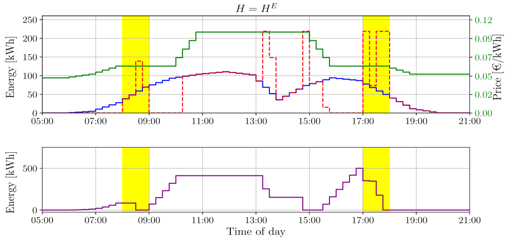
Fig. 3. Example 1. Results for Entity 1 on day 24 under Problem 2 with H = H^E . Energy production forecast \hat{E}_a(t) (blue), sold energy E_s^e(t) (dashed red), energy selling price \pi_a^e(t) (green), storage energy level S_a(t) (purple), and time periods of DR requests (yellow). (For interpretation of the references to color in this figure legend, the reader is referred to the web version of this article.)
